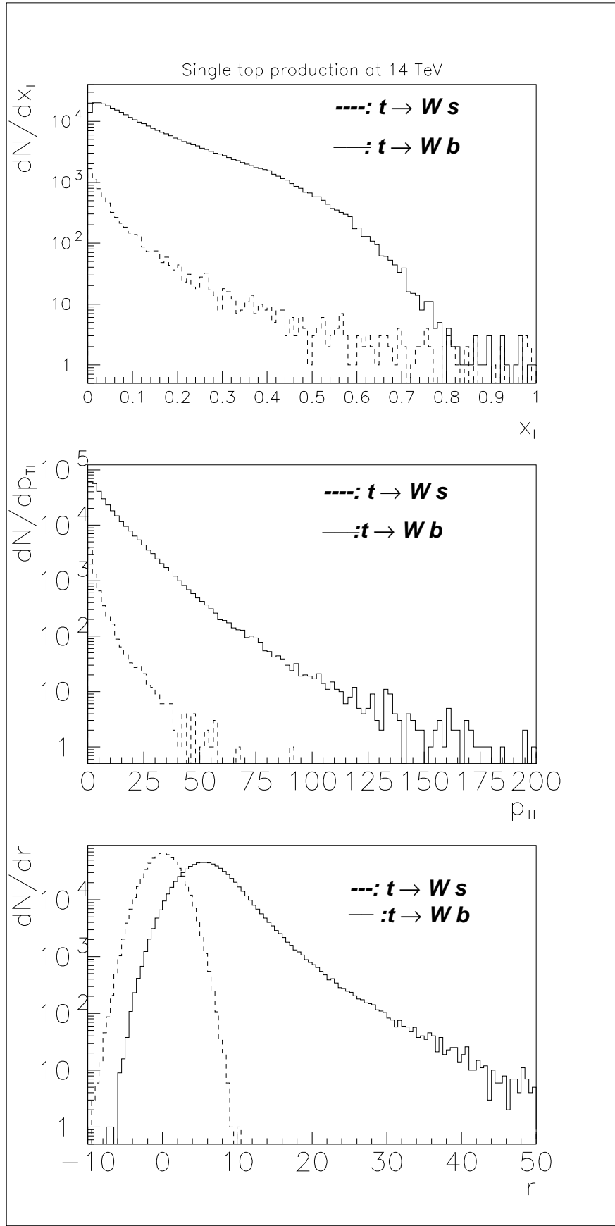
FIG. 5: pp \rightarrow t/\bar{t}X at \sqrt{s} = 14 TeV. Upper frame: scaled- \ell^\pm -energy distributions, dN/dx_\ell , from t \rightarrow W s ( \rightarrow \ell^\pm X ) (lower histogram) and t \rightarrow W b ( \rightarrow \ell^\pm X ) (upper histogram). Middle frame: Transverse momentum distributions of the \ell^\pm s measured w.r.t. beam axis dN/dp_{T\ell} (in GeV), in the same production and decay processes as in the upper frame. Lower frame: Secondary decay vertex distributions in the variable r (in millimetres) for the two decay chains t \rightarrow W s (solid histogram) and t \rightarrow W b (dashed histogram) obtained
