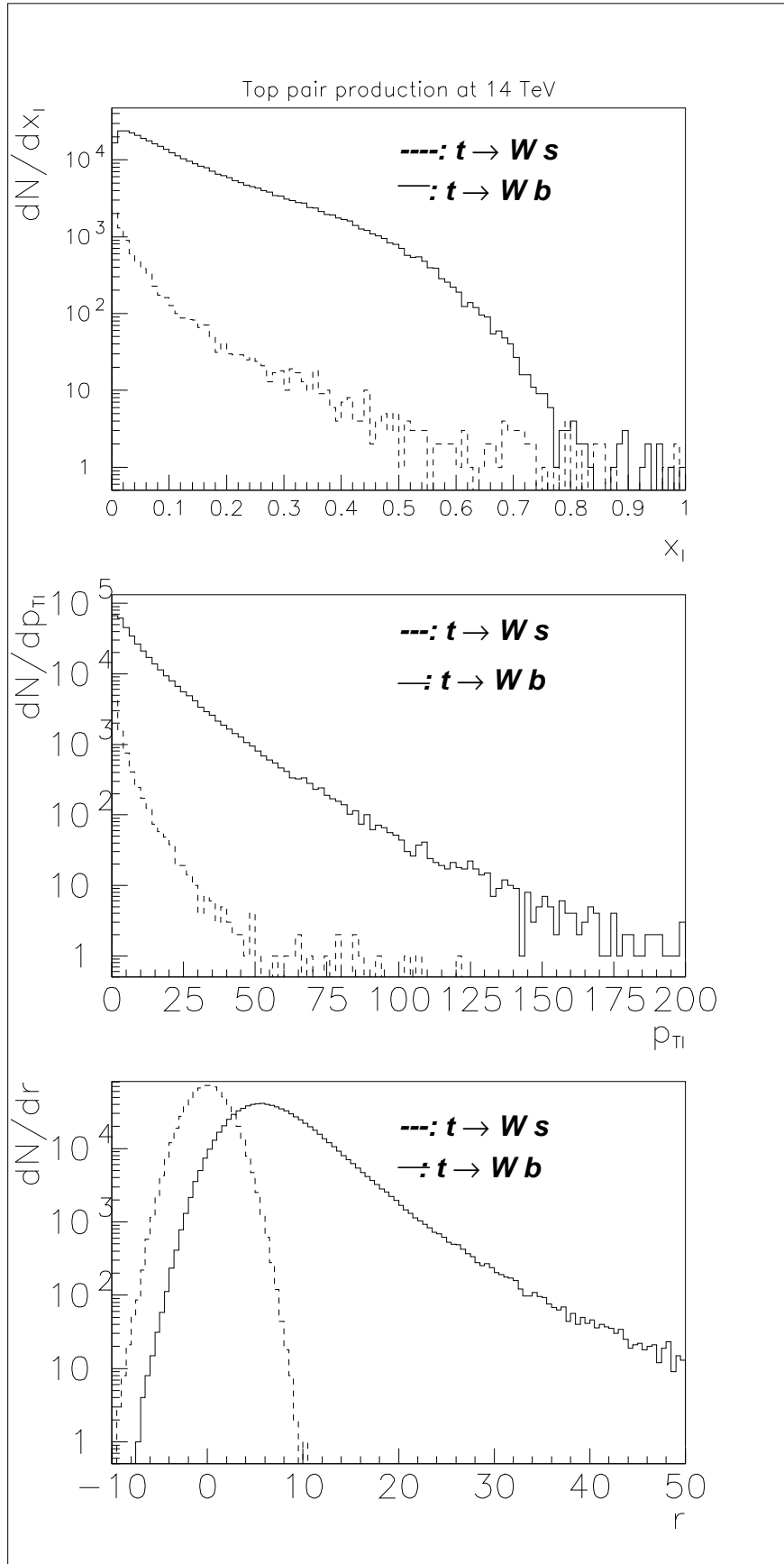
FIG. 2: pp \rightarrow t\bar{t}X at \sqrt{s} = 14 TeV. Upper frame: scaled- \ell^\pm -energy distributions, dN/dx_\ell , from t \rightarrow W s ( \rightarrow \ell^\pm X ) (lower histogram) and t \rightarrow W b ( \rightarrow \ell^\pm X ) (upper histogram). Middle frame: Transverse momentum distributions of the \ell^\pm s measured w.r.t. beam axis, dN/dp_{T\ell} (in GeV), in the same production and decay processes as in the upper frame. Lower frame: Secondary decay vertex distributions in the variable r (in
